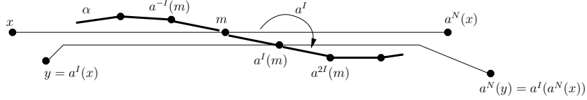
Fig. 1. Two geodesics [x, a^N(x)] and [y, a^N(y)] stay 2\delta -close for the most part. The geodesic [m, a^I(m)] is “pinched” between those two geodesics.
