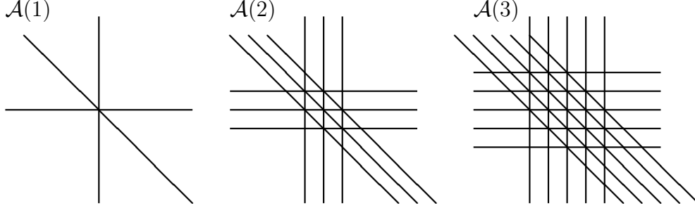
Figure 1: Example of A_2 -type arrangements
